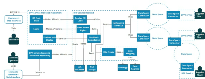
Figure 1: The initial architecture of the DPP system provides a detailed overview of the DPP service frontend for customers and the DPP service backend. Other components are presented at a higher level to offer a broader view of the entire DPP system. The architecture is formalized using the C4 model.
